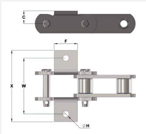
K1 Attachments
