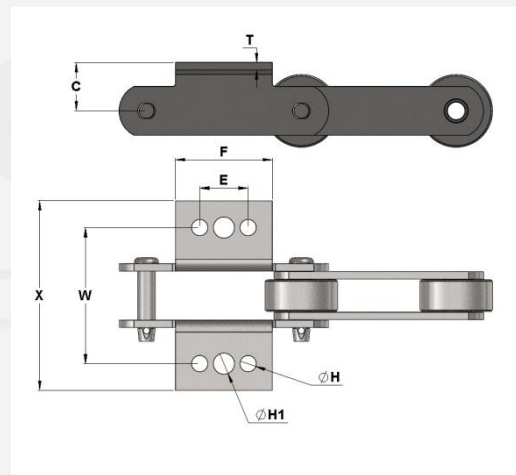
K3 Attachments
