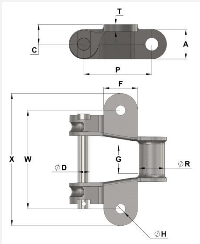
K1 Attachment
