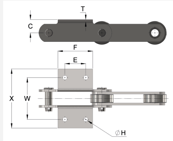
K2 Attachments
