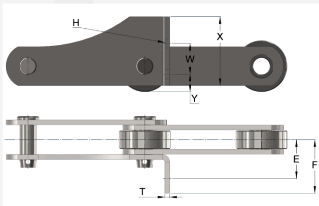
LA 2 Attachments
